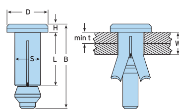
b) Countersunk
