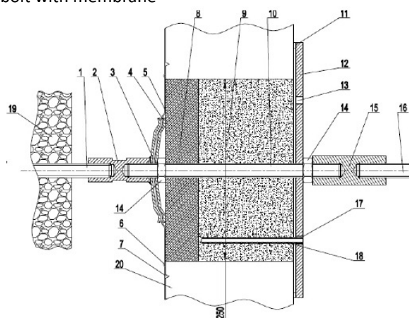
PTC-223-2 Water stop technical bolt with membrane
