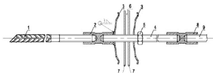
PTC-076-3 Water stop rebar bolt, ceiling-version 2
