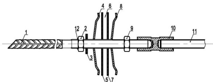
PTC-076-1 Water stop rebar bolt, ceiling-version 1
