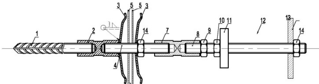
PTC-076-4 Water stop rebar bolt, wall
