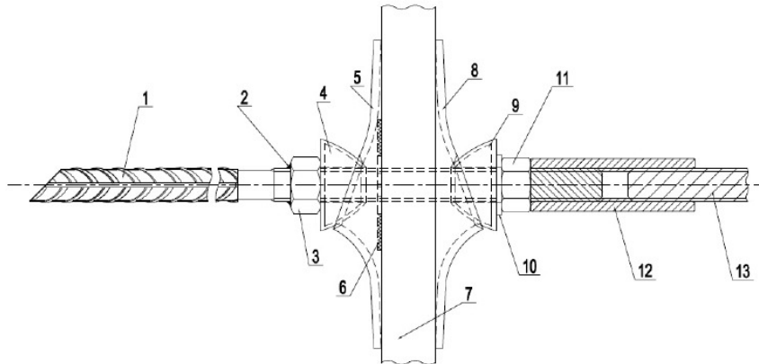
PTC-076-15 Water stop technical bolt, M20/M24
