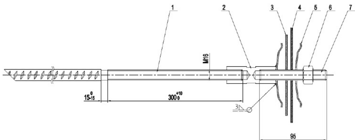
PTC-076-16 Water stop bolt for membrane M16
