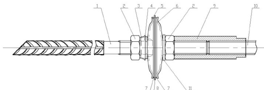
PTC-076-12 Water stop rebar bolt M33, version 3
